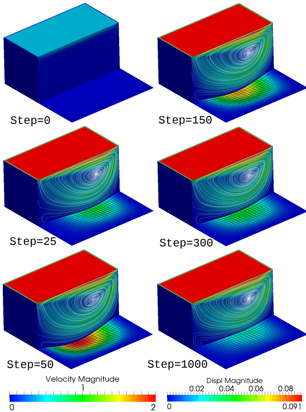
Figure 8: Fluid Velocity, plate displacement and streamlines .
