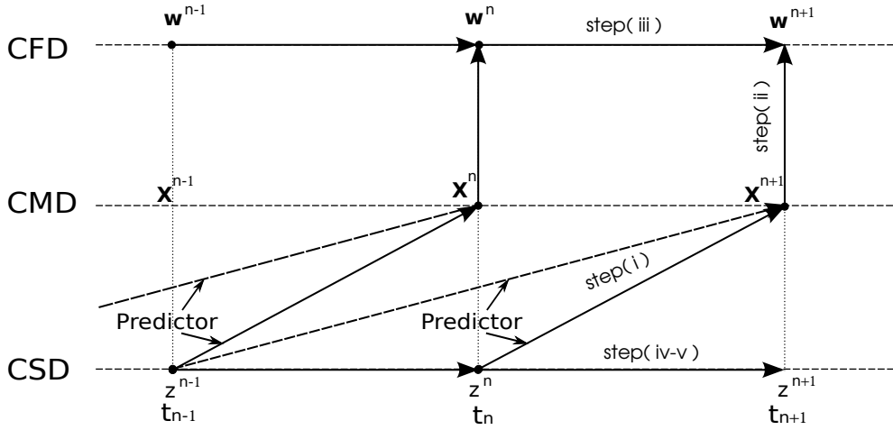
Figure 1: Weak coupling scheme.
