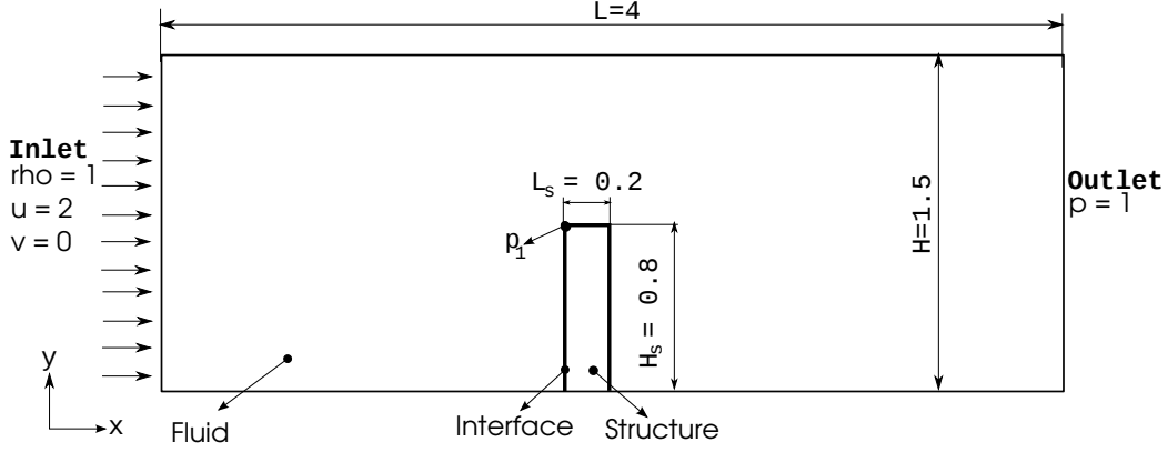
Figure 3: Fluid domain and dimensions.
