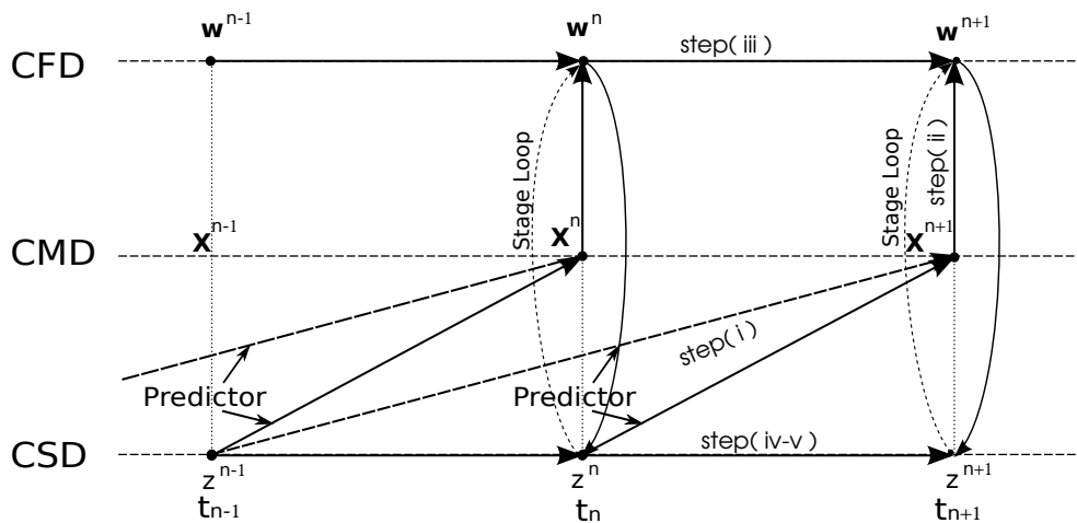
Figure 2: Strong coupling scheme.
