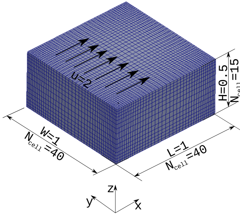
Figure 6: 3D Lid-driven cavity.
