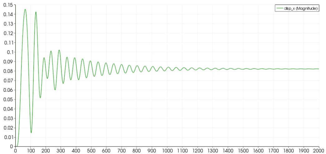
Figure 4: Magnitude of the displacement at point 1.
