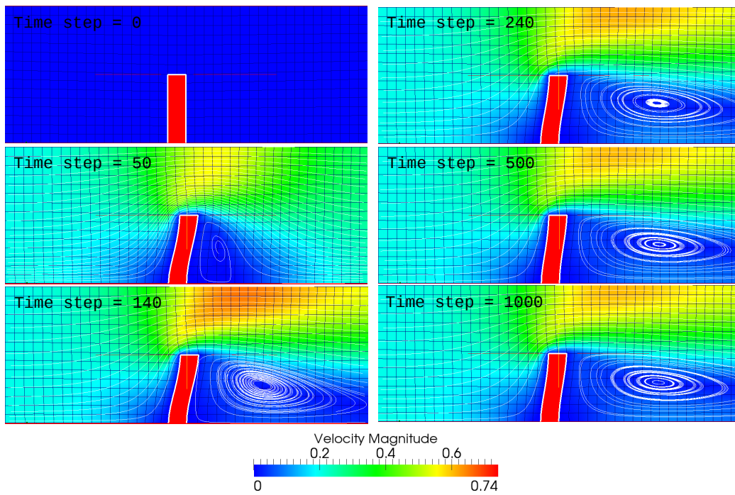
Figure 5: Deformations of the beam and streamlines for time steps \{0, 50, 140, 240, 500, 1000\} .
