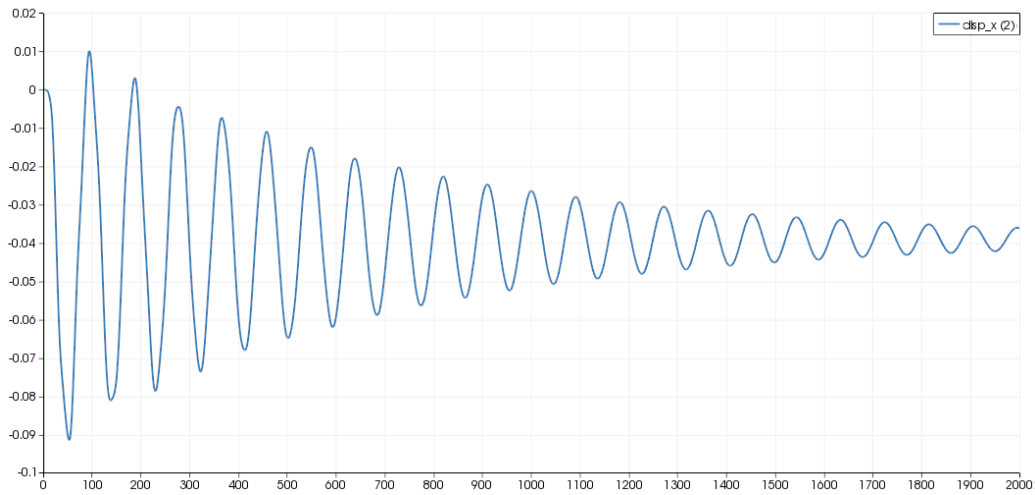
Figure 7: Displacement Magnitude at the middle of the plate.
