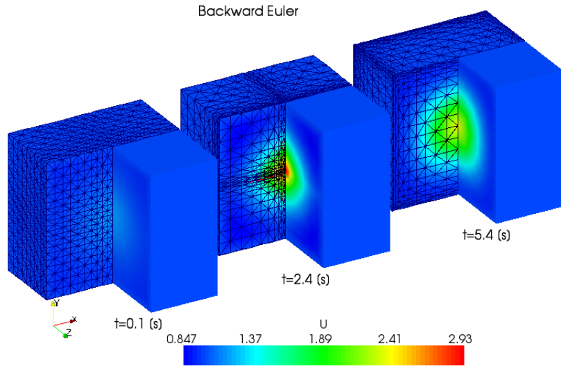
Figure 11: Solution for the Backward Euler (BE) scheme.
