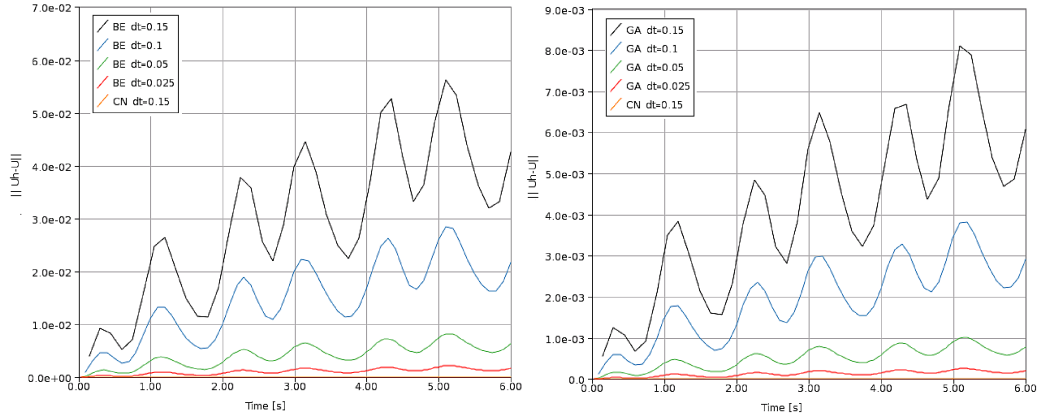
Figure 2: \|u_h - u\|_{L^2(\Omega^n)} for Garlerkin (GA) and Backward Euler (BE) schemes compared with Crank-Nicolson (CN).
