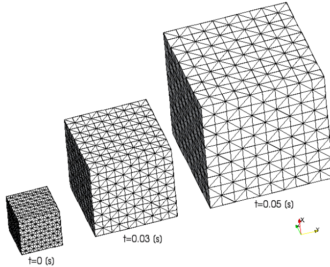
Figure 7: Deformed domain.
