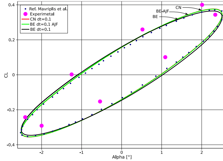
Figure 13: Lift coefficient as a function of the angle of attack for \Delta t = 0.1[s] .
