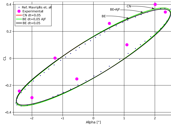
Figure 14: Lift coefficient as a function of the angle of attack for \Delta t = 0.05[s] .
