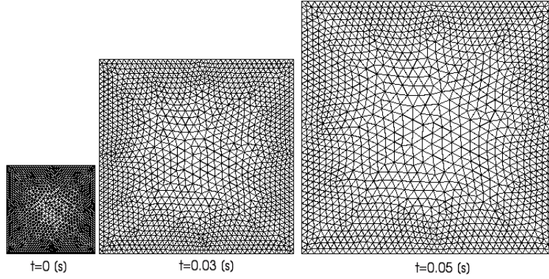
Figure 5: Deformed domain.
