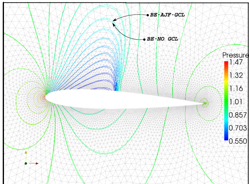
Figure 15: Comparison of isobars for \alpha = 2.51^\circ .
