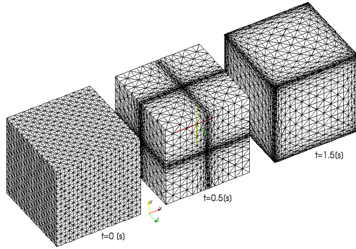
Figure 9: Deformed mesh.
