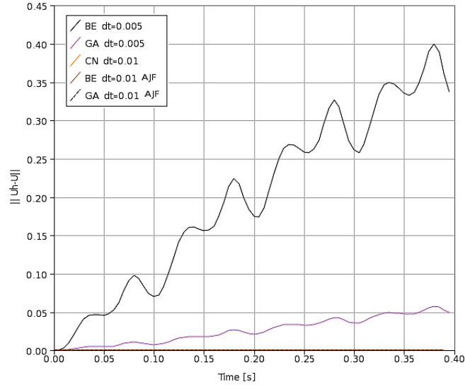
Figure 6: \|u_h - u\|_{L^2(\Omega^n)} for Backward Euler (BE), Galerkin (GA) and Crank-Nicolson (CN) schemes.
