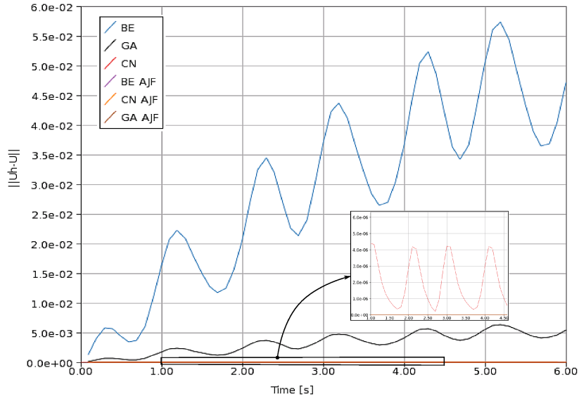
Figure 10: \|u_h - u\|_{L^2(\Omega^n)} for Backward Euler (BE), Galerkin (GA) and Crank-Nicolson (CN) schemes.
