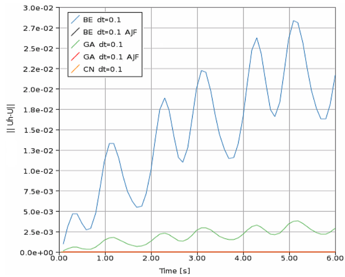
Figure 4: Errors for Averaged Jacobian Formulation (AJF) and No-Averaged Jacobian Formulation.
