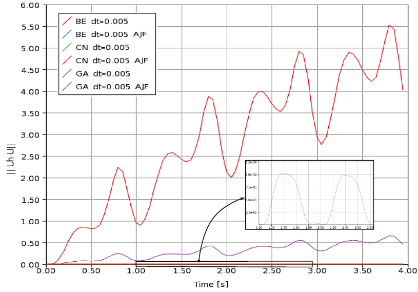
Figure 8: Errors for Averaged Jacobian Formulation (AJF) and No-Averaged Jacobian Formulation.
