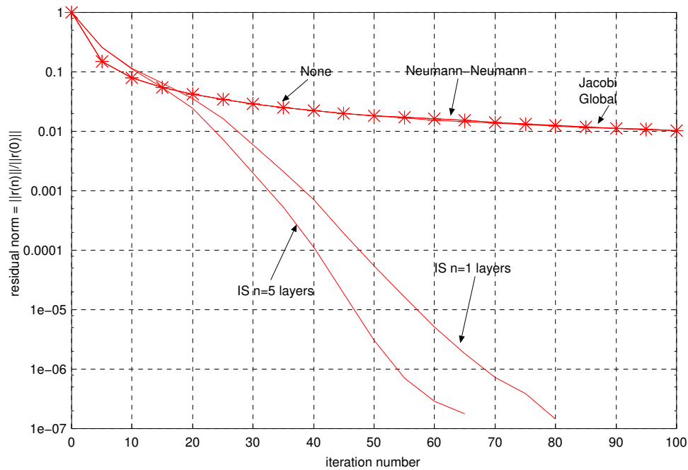
Figure 9. Iteration counts for advective-diffusive problem ( mesh 1000 \times 1000 ).
