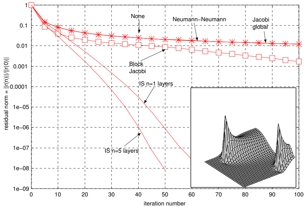
Figure 8. Solution of advective-diffusive problem ( mesh 500 \times 500 ).
