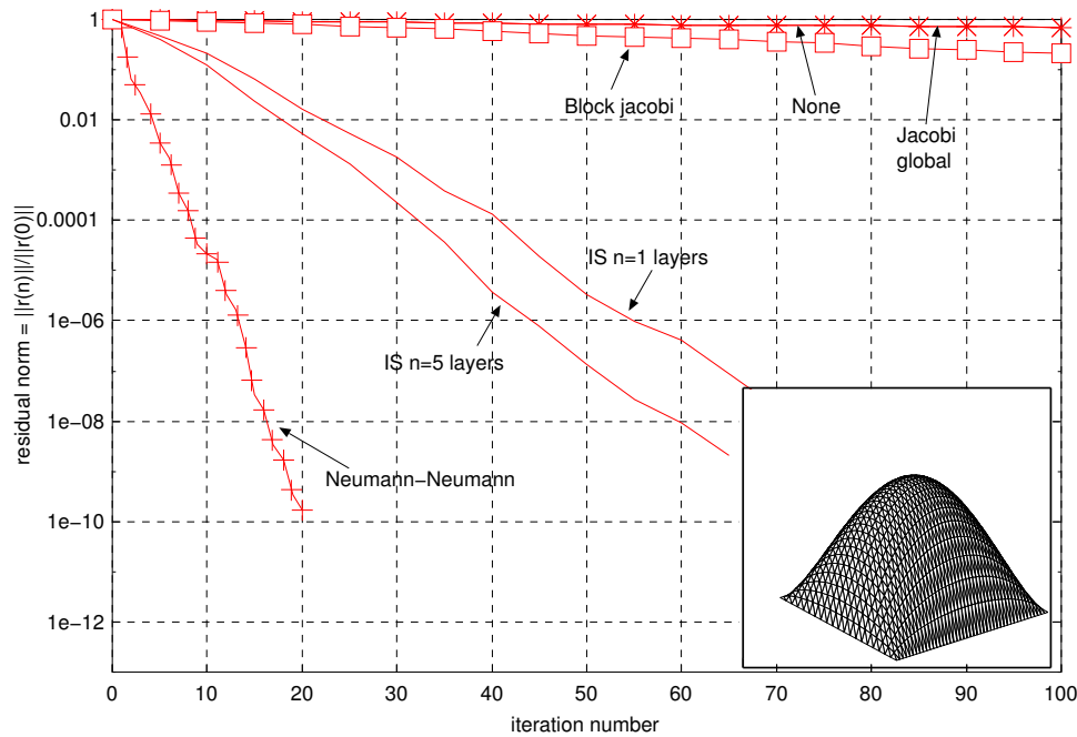
Figure 7. Solution of Poisson's problem ( mesh\ 500 \times 500 ).
