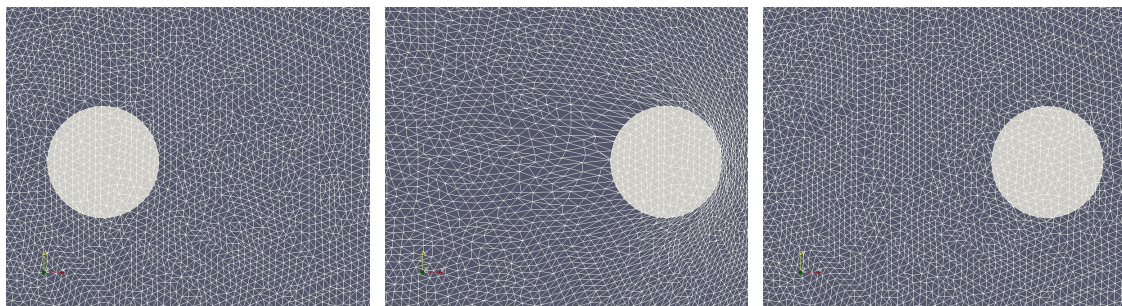
(a) Body-fitted mesh obtained from the reference mesh. (b) Deformed body-fitted mesh after some time steps. (c) New body-fitted mesh obtained from the reference mesh after performing the reset and readjustment step.
