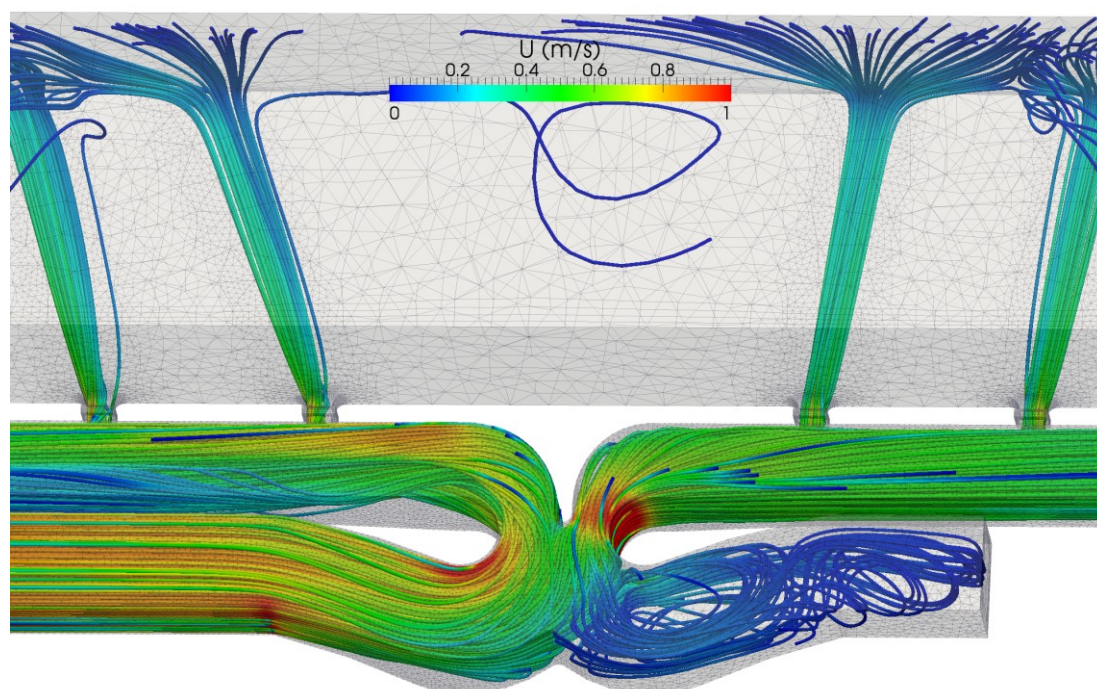
Figure 12: Streamlines for Central Connection
