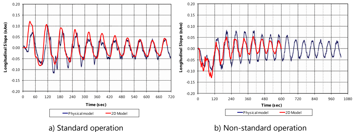
Figure 4: Validation of 2D model: longitudinal water slope at Chamber, for Lock to Lock operation
