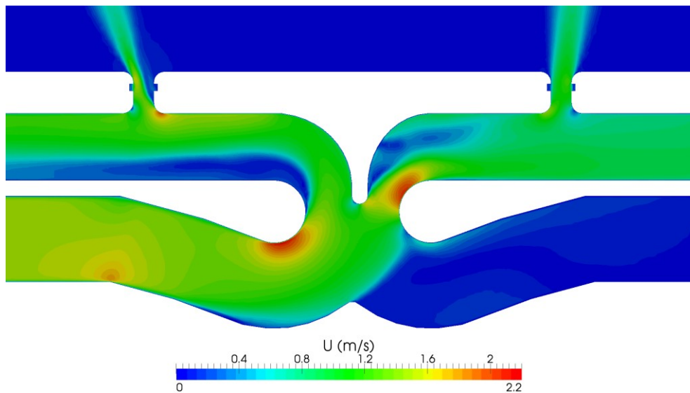
Figure 15: Velocity distribution according to Numerical Scaled Model
