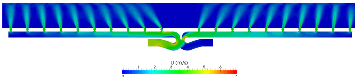
Figure 11: Plan view of velocity distribution for Central Connection
