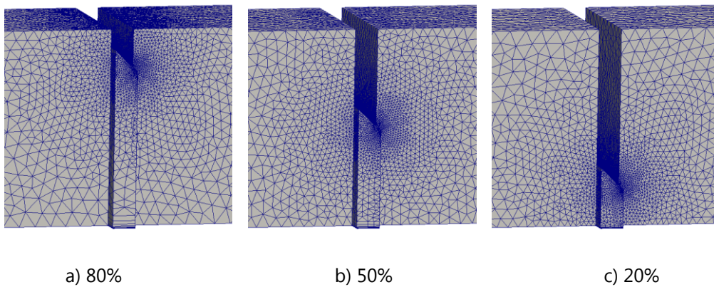
Figure 8: Detail of mesh for the different valve apertures
