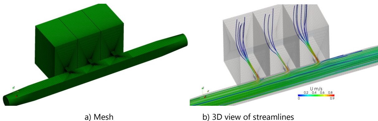
Figure 6: Validation of 3D model with port system problem
