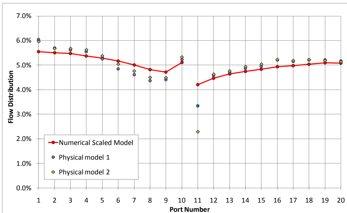
Figure 14: Flow distribution among ports according to physical model and Numerical Scaled Model
