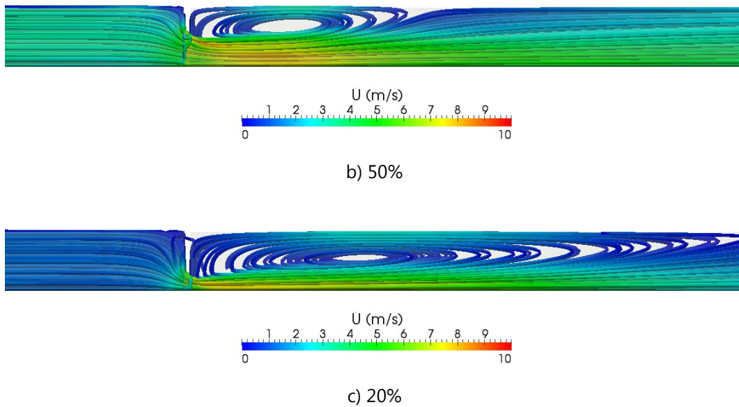
Figure 9: Streamlines and velocity for the different valve apertures
