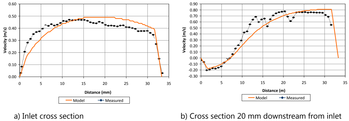
Figure 7: Velocity profiles at mid-plane of ports.
