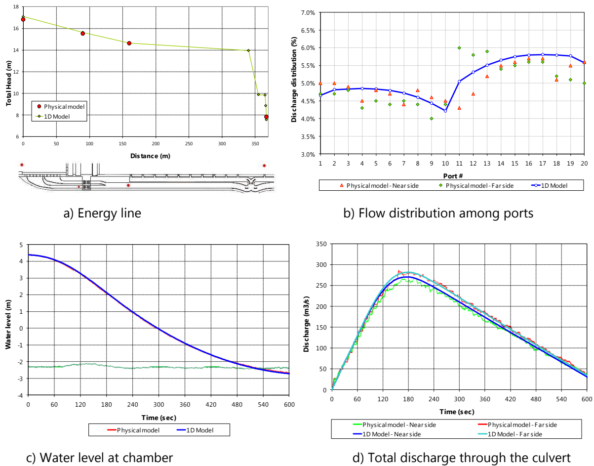
Figure 3: Validation of 1D model
