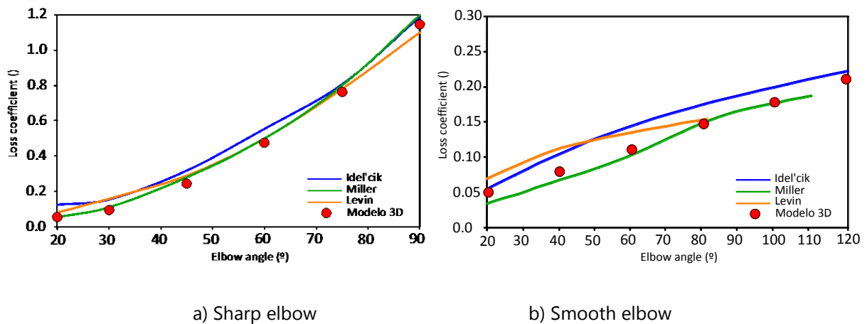
Figure 5: Validation of 3D model with elbow problem
