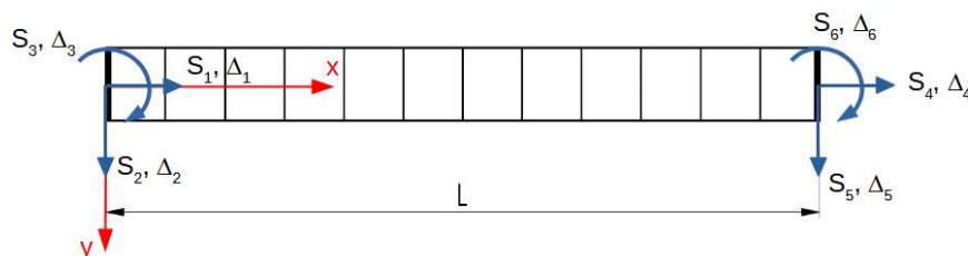
Figure 1: Beam model
