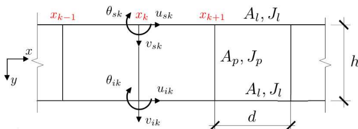
Figure 2: Beam sector
