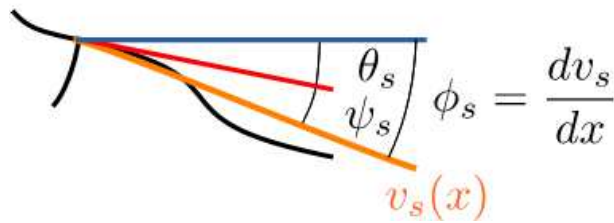
Figure 4: Nodal rotations
