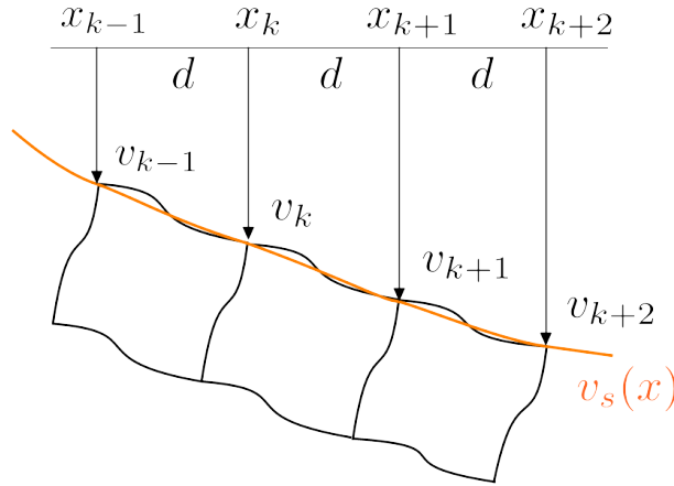
Figure 3: Shear distortion
